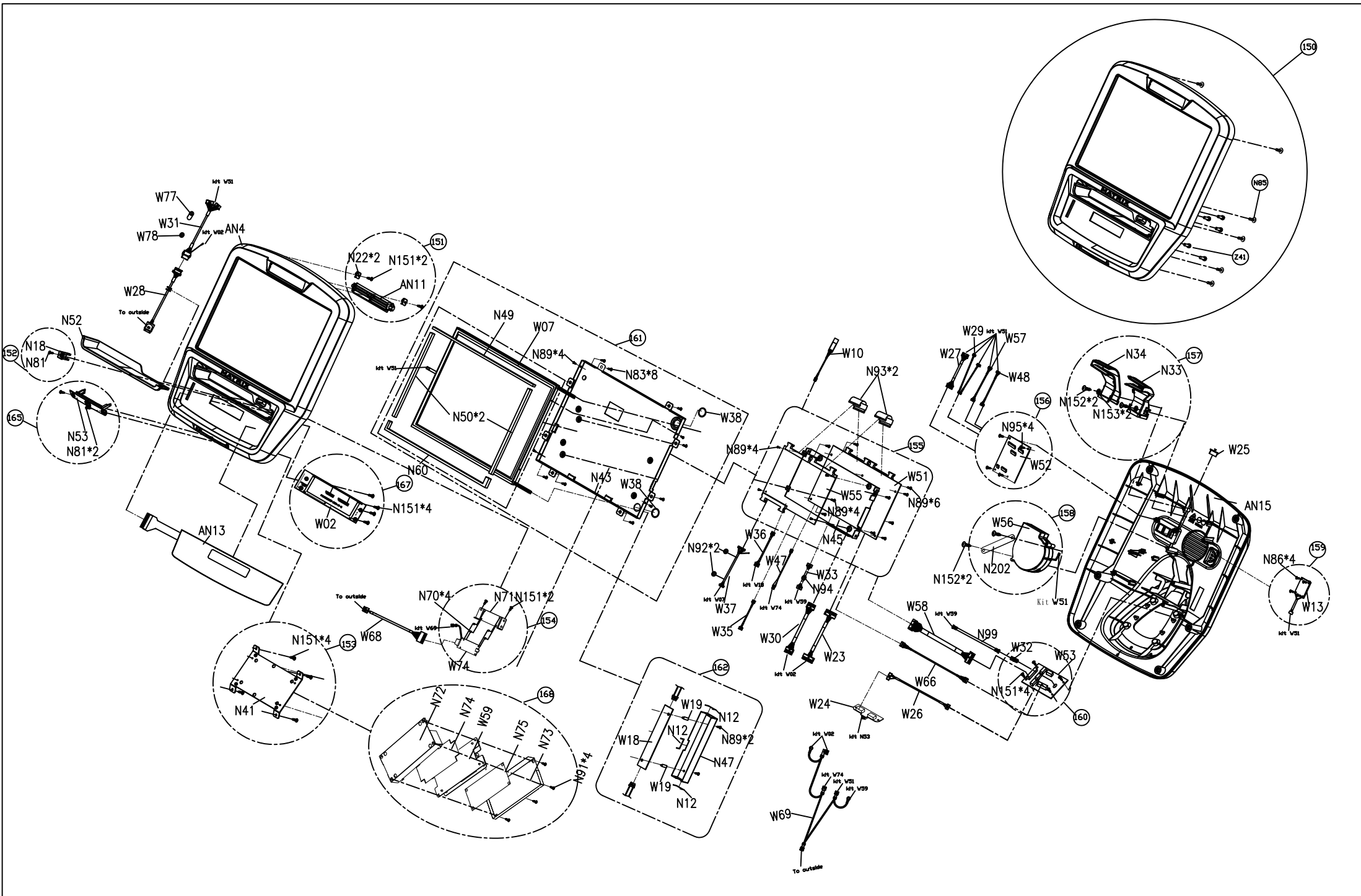
Service drawing of matrix H7XE / U7XE / R7XE / E7XE / S7XE / A7XE console
